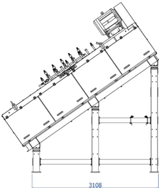
Paddle Washer |
