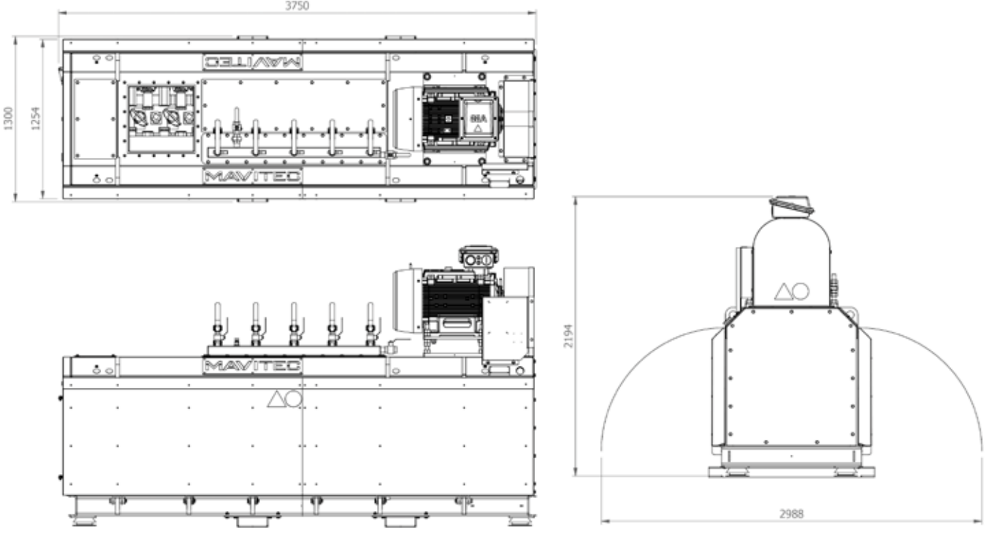
Paddle Depacker†
