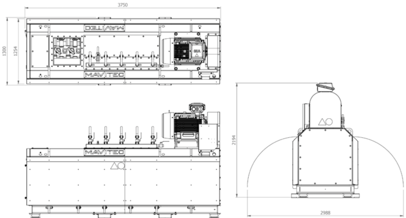
Paddle Depacker†
