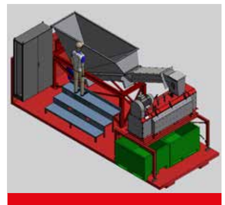
Mavitec's Paddle Depacker Model S as a containerized solution with a small footprint.
